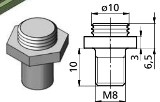
PRG1003M8
