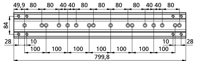
ACB4050800 kg ~35
